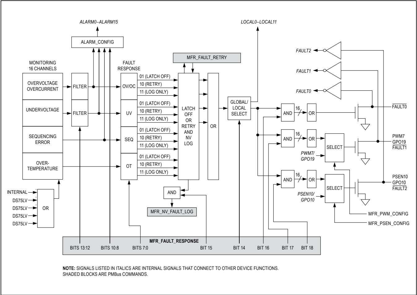
Figure 10. MFR_FAULT_RESPONSE Operation
